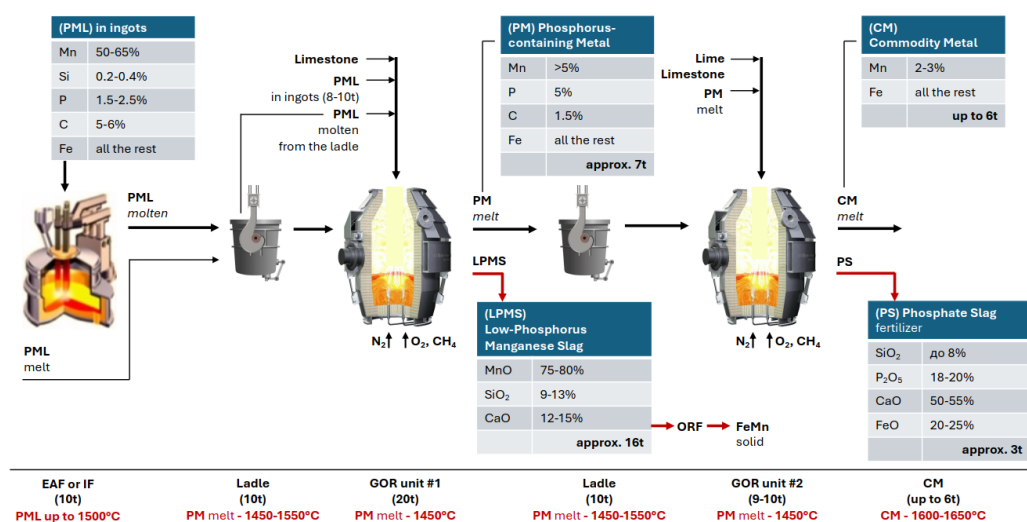
The technological flow chart for processing of phosphorus-containing manganese ligature (PML)
